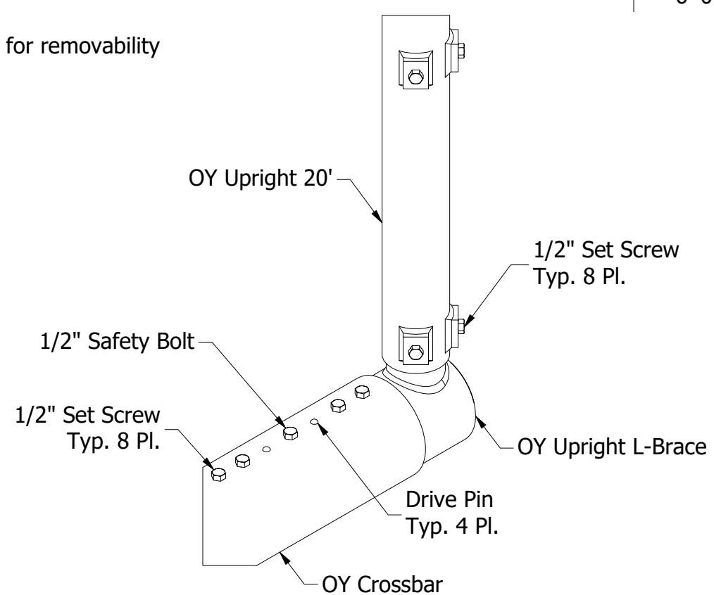
DETAIL A CROSSBAR
