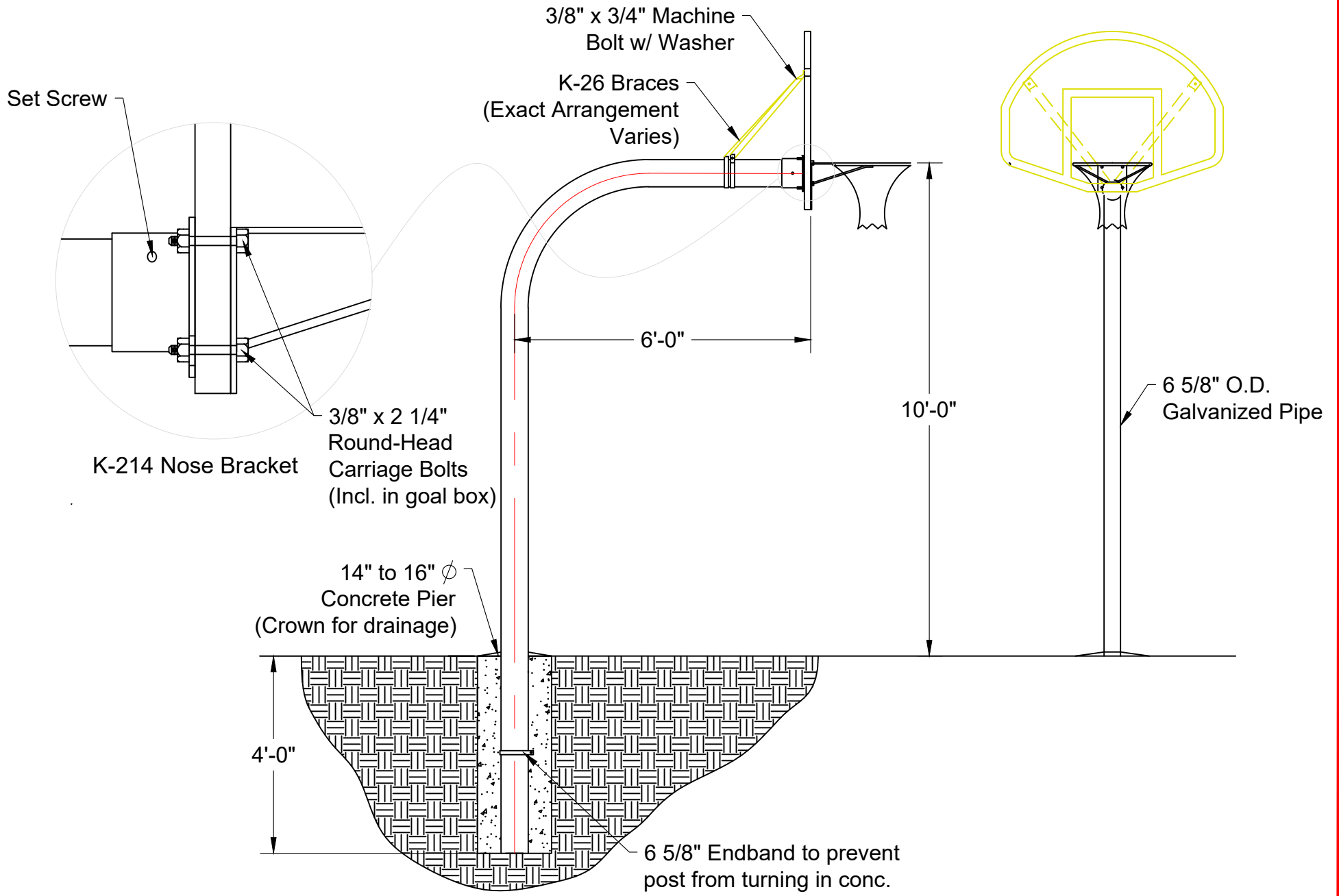
MODEL #G66 SCALE: 3/8"=1'-0"
